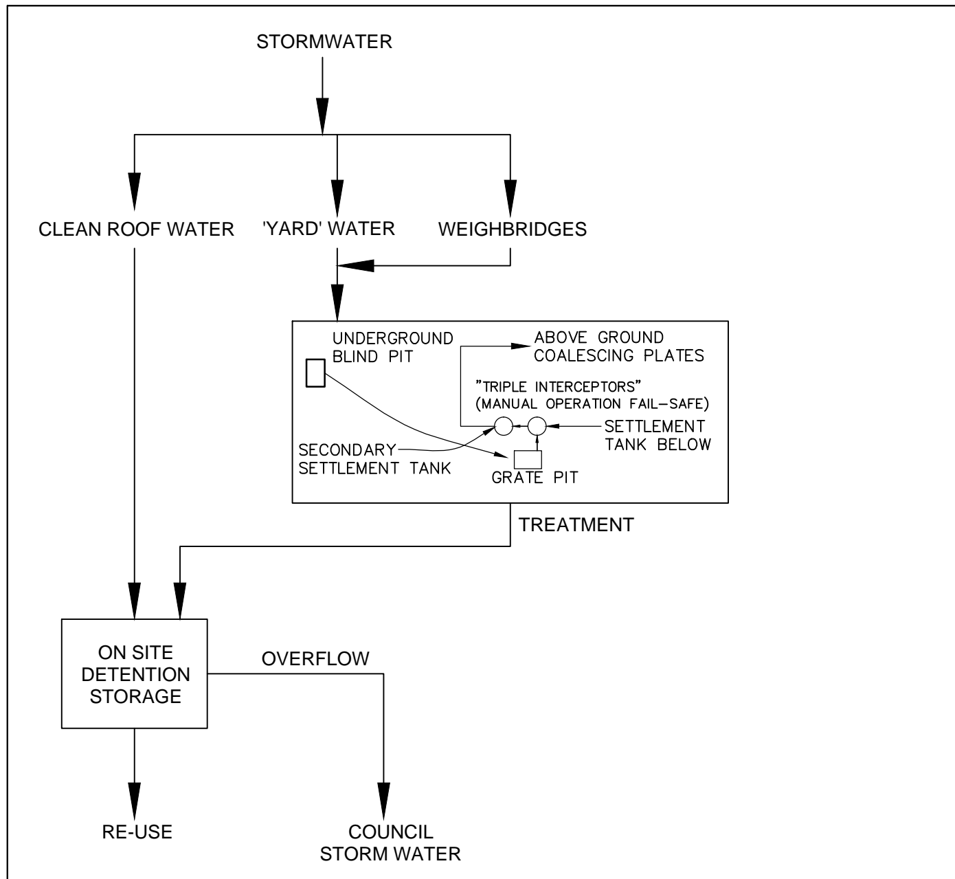
② PROPOSED WATER CYCLE SCHEMATIC
